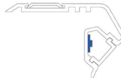
LED Strip
