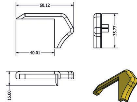
PI_0214 FLAT END CAP (LEFT AND RIGHT)
