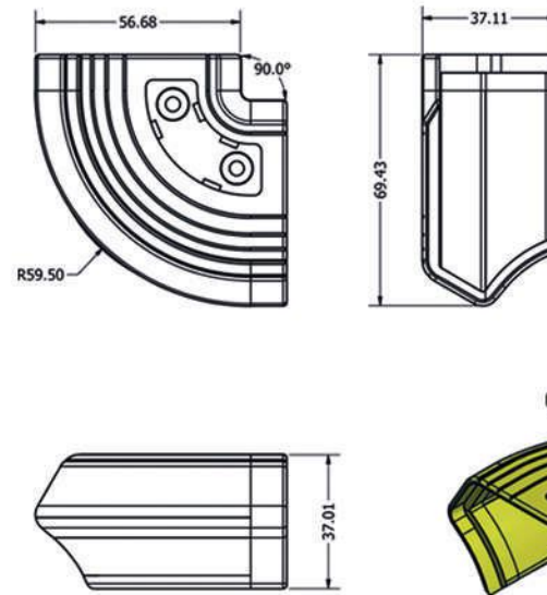
AP_0139 CONCAVE CORNER PLASTIC PART
