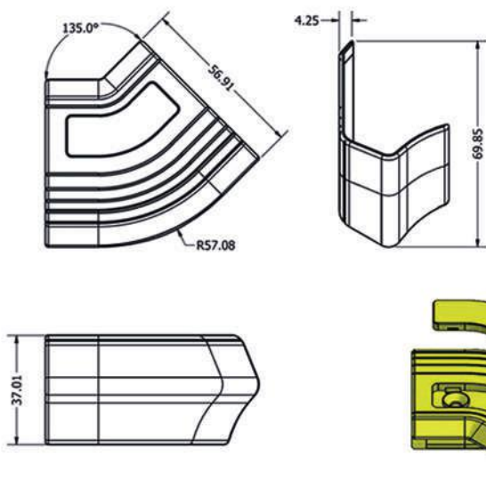
AP_0140 CONVEX CORNER PLASTIC PART
