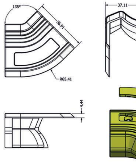
AP_0139 CONCAVE CORNER PLASTIC PART
